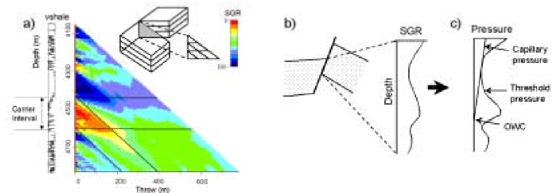
Fig. 1. Schematic diagram illustrating the method of calculation of fault seal capacity. (a) Sequence-throw juxtaposition diagram constructed for the vshale curve on the left of the figure (TVD in metres) and contoured for SGR. The horizontal and diagonal lines are the top and base of the carrier interval on the upthrown and downthrown side of the fault, respectively. The diagram construction is illustrated in the inset. In the inset, the stippled area represents the carrier interval. The SGR versus depth curve for the relevant fault trace segment (b) is converted to a threshold pressure curve (c). The depth of the oil-water contact is determined by the minimum capillary pressure due to buoyancy required to intersect the fault threshold pressure curve.
