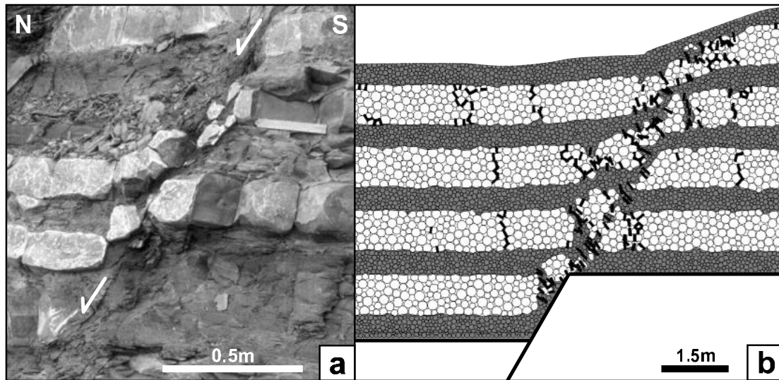
Figure 1: (a) Normal fault in Jurassic limestone/shale sequence at Kilve foreshore, Somerset, UK. (b) Normal fault in distinct element model of interbedded strong (white) and weak (grey) layers. Bold lines indicate broken bonds.
